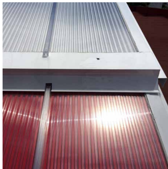
CIIDET College & University, Mexico | Glazing: Danpalon 3DLITE | IIFEQ Architects
