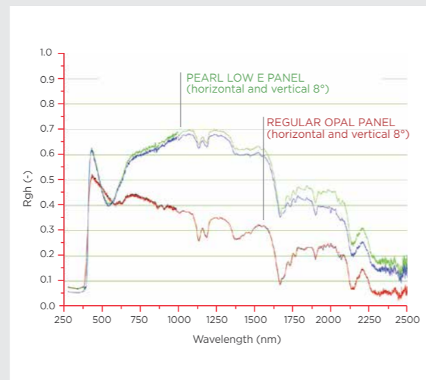
"PEARL LOWE" has improved IR reflectivity characteristics, compared to a similar panel without infrared treatment (as shown in the graph).
